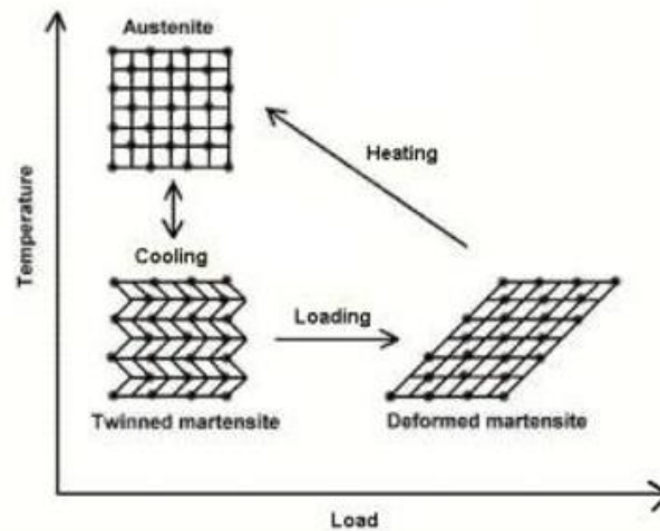
Figure 3: Material Phenomena
